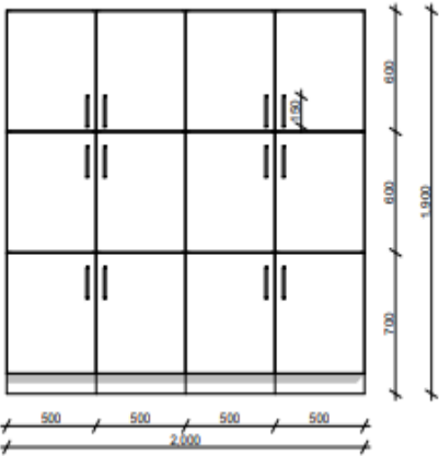
Elevations
