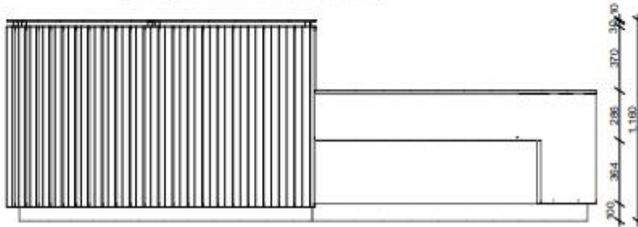
Reception Desk Elevation
